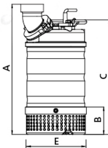
80EUB-5.20M~5.75M
