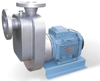
INDUSTRIAL SELF-PRIMING CENTRIFUGAL PUMP FL90CAI
